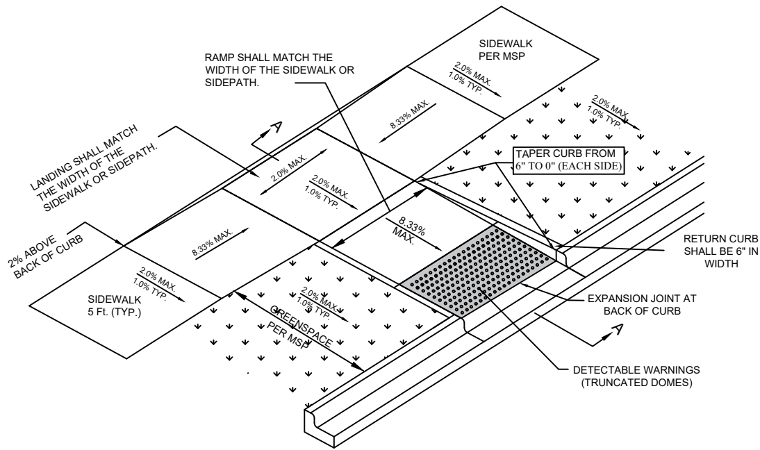
RETURN CURB RAMP PLAN VIEW
