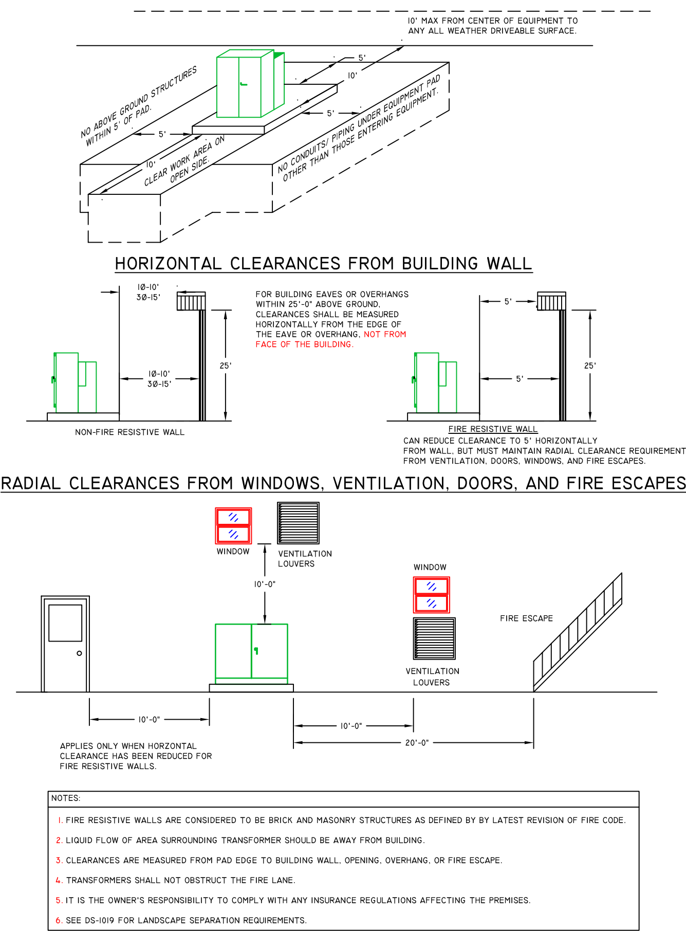
DS-I410 CLEARANCE SPECIFICATIONS FOR PADMOUNTED EQUIPMENT
